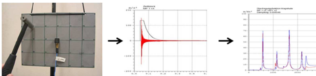
Fig 6 Frequency Measurement, Impact-Hammer-Method
