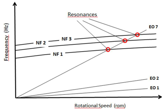
Fig 4 Campbell-Diagram (Principle)
