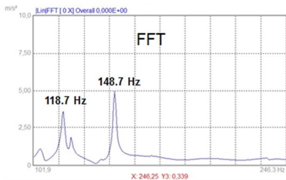
Fig 10 Frequency analysis of the damaged blade
