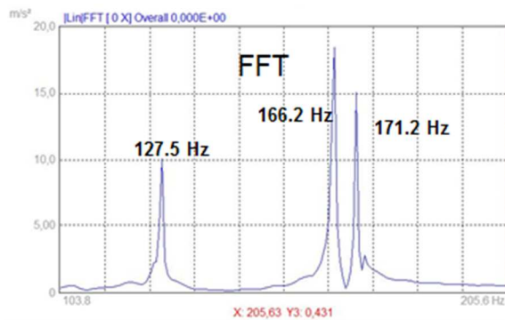
Fig 9 Frequency analysis of the undamaged blade
