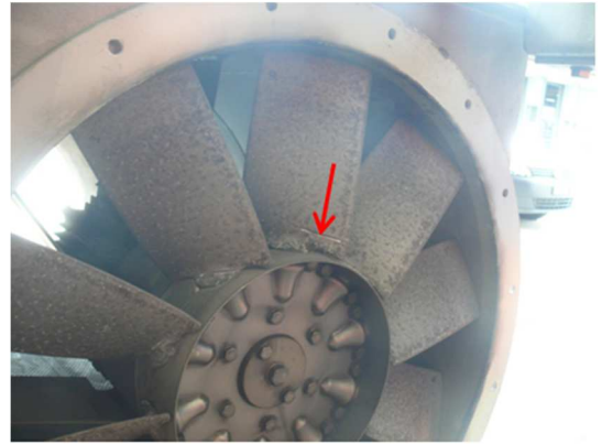
Fig 8 Damaged blade with a partial cut
