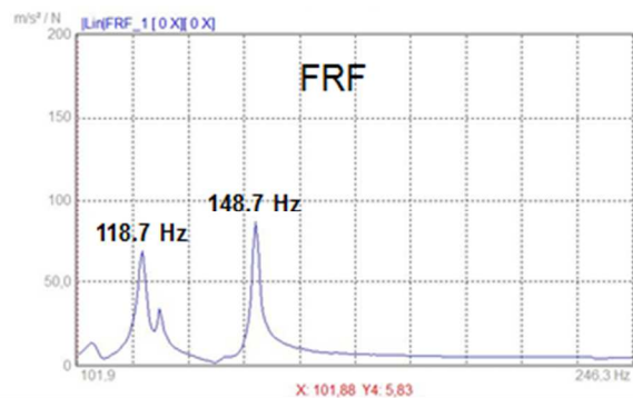
Fig 10 Frequency analysis of the damaged blade
