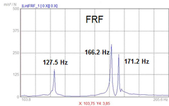
Fig 9 Frequency analysis of the undamaged blade
